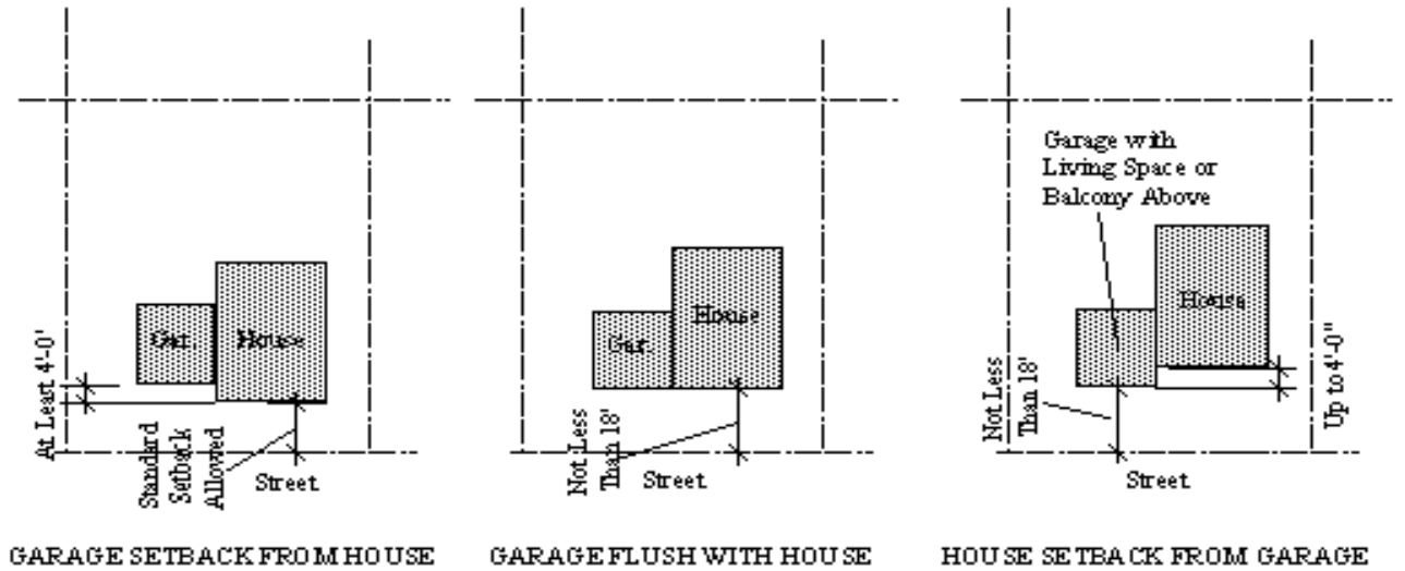
Figure A12.004 – Front Yard Setbacks
